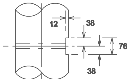
DETAIL D SCALE 1:10
